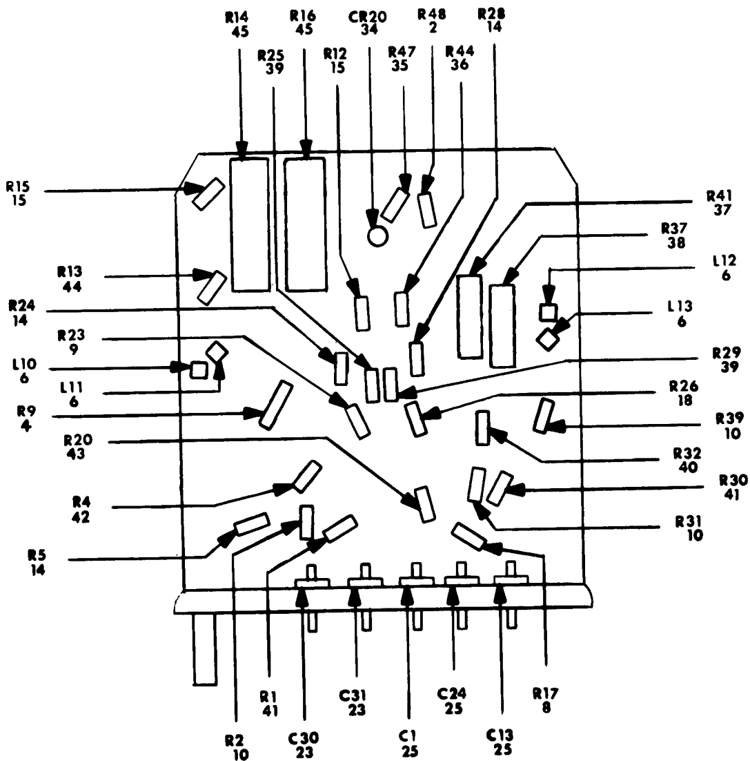
Figure 2-9. Module M19H (Sheet 4 of 7).
