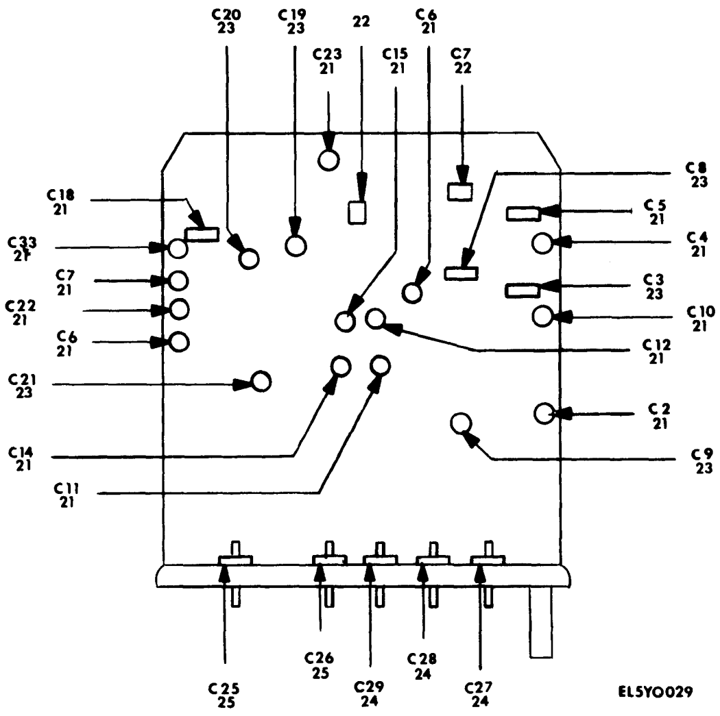
Figure 2-9. Module M19H (Sheet 2 of 7).
