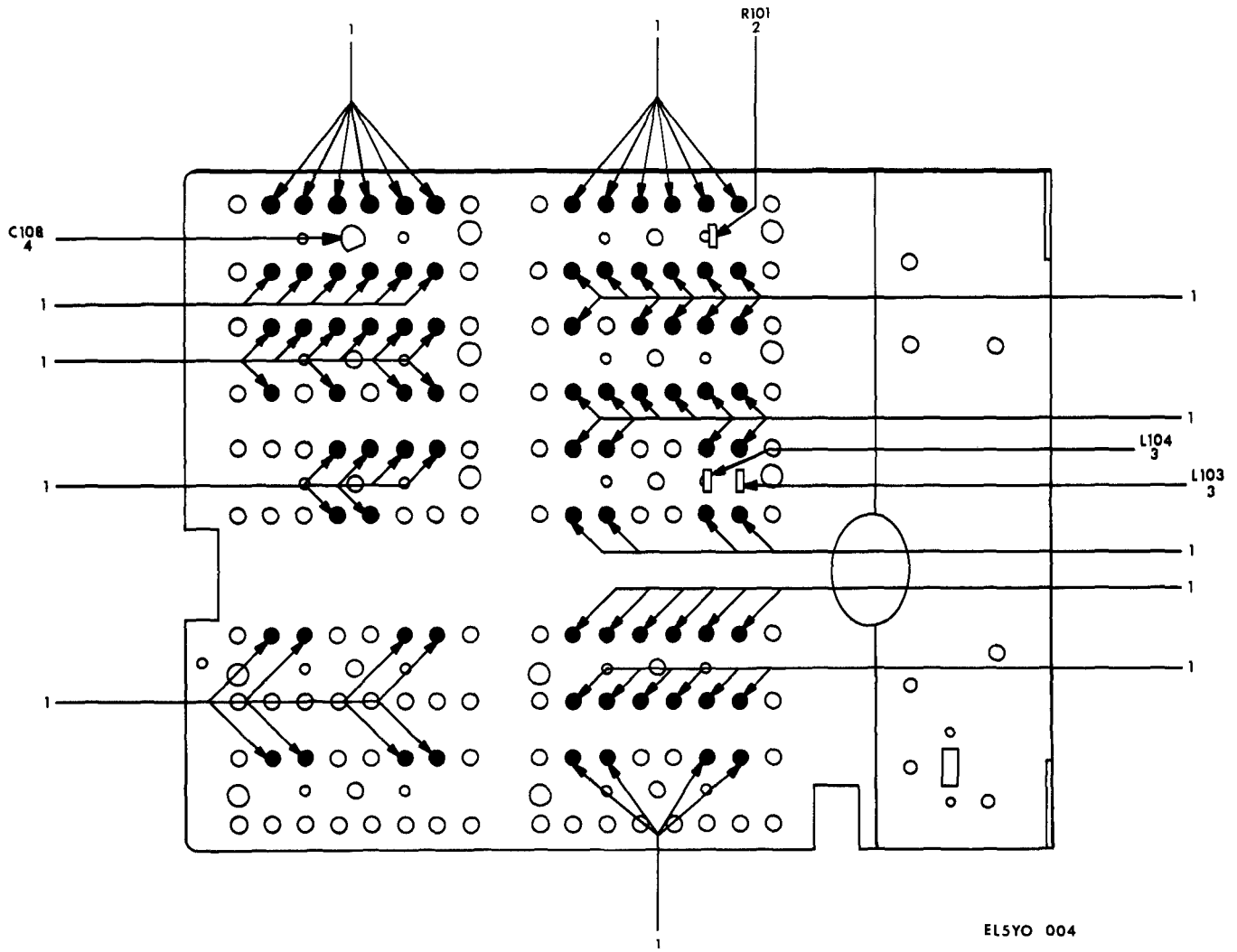
Figure 2-3. Sweep Generator SG-677A/U, Chassis Assembly, (Sheet 1 of 6).
