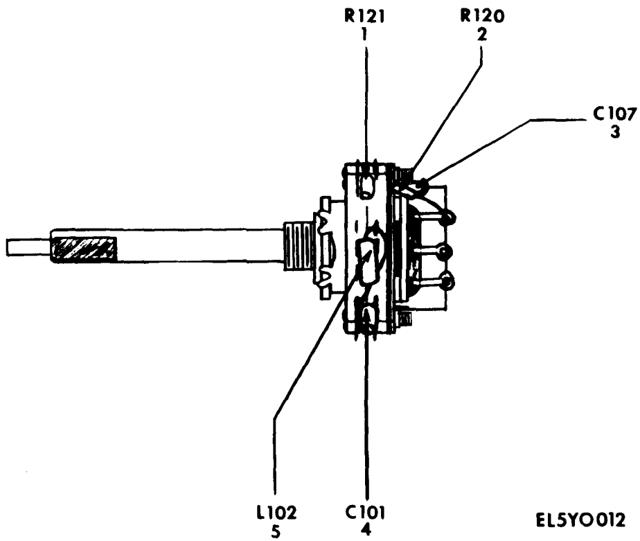
Figure 2-5. Sweep Generator SG-677A/U, Marker Size Switch Assembly (Sheet 1 of 2).
