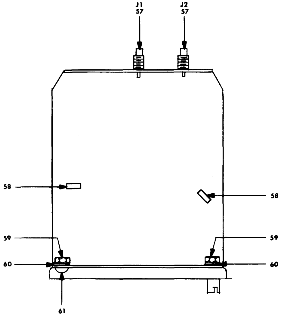
Figure 2-7. Module M9H (Sheet 5 of 5).
