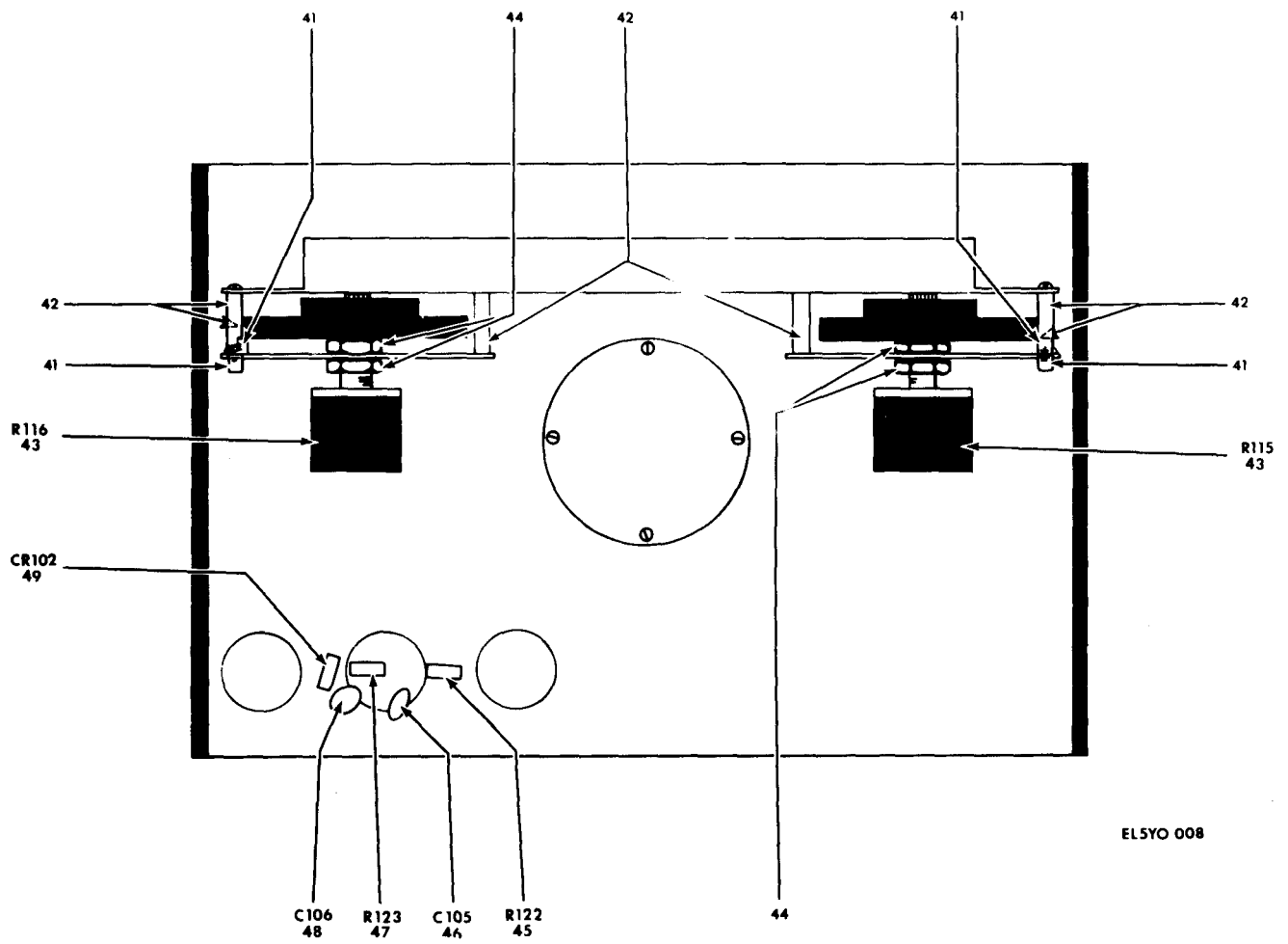
Figure 2-3 Sweep Generator SG-677A/U, Chassis Assembly, (Sheet 5 of 6).
