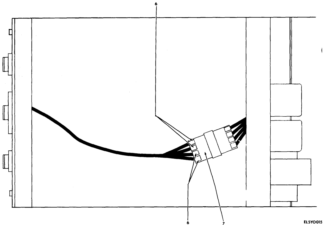
Figure 2-6. Sweep Generator SG-677A/U, Harness Assembly (Sheet 2 of 2).
