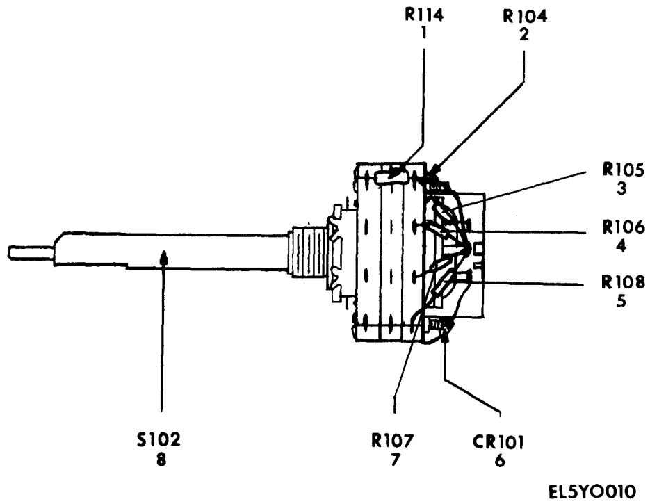
Figure 2-4. Sweep Generator SG-677A/U, Sweep Time Switch Assembly (Sheet 1 of 2).
