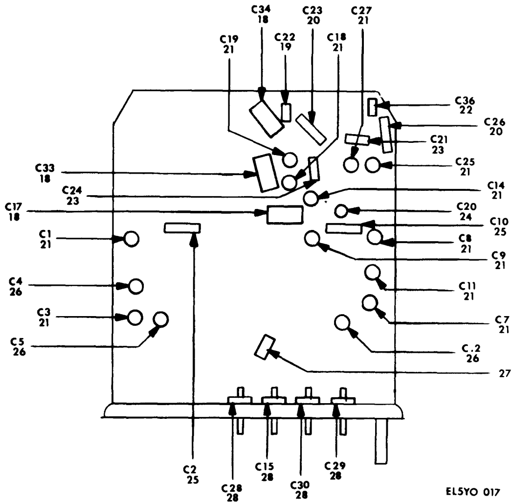
Figure 2-7. Module M9H (Sheet 2 of 5).
