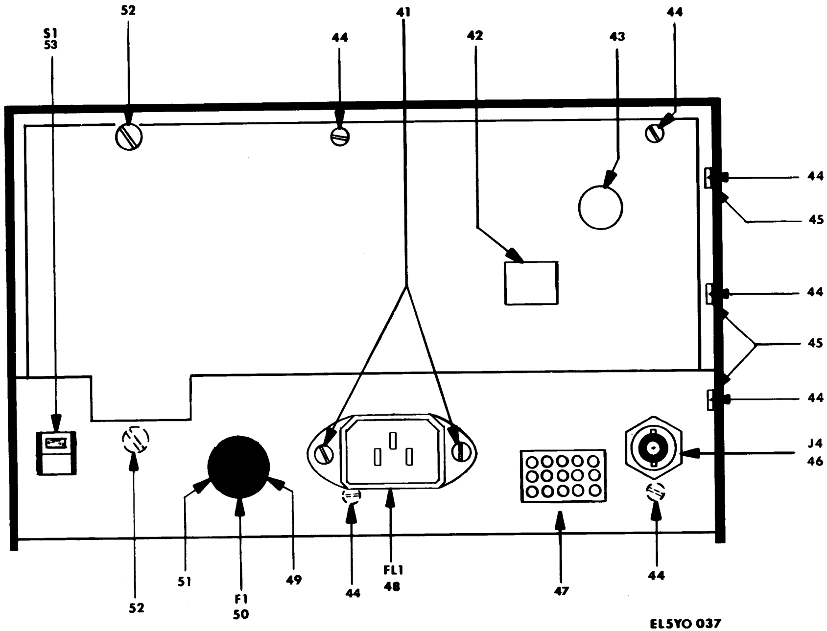
Figure 2-10. Power Supply PS6A (Sheet 3 of 4).
