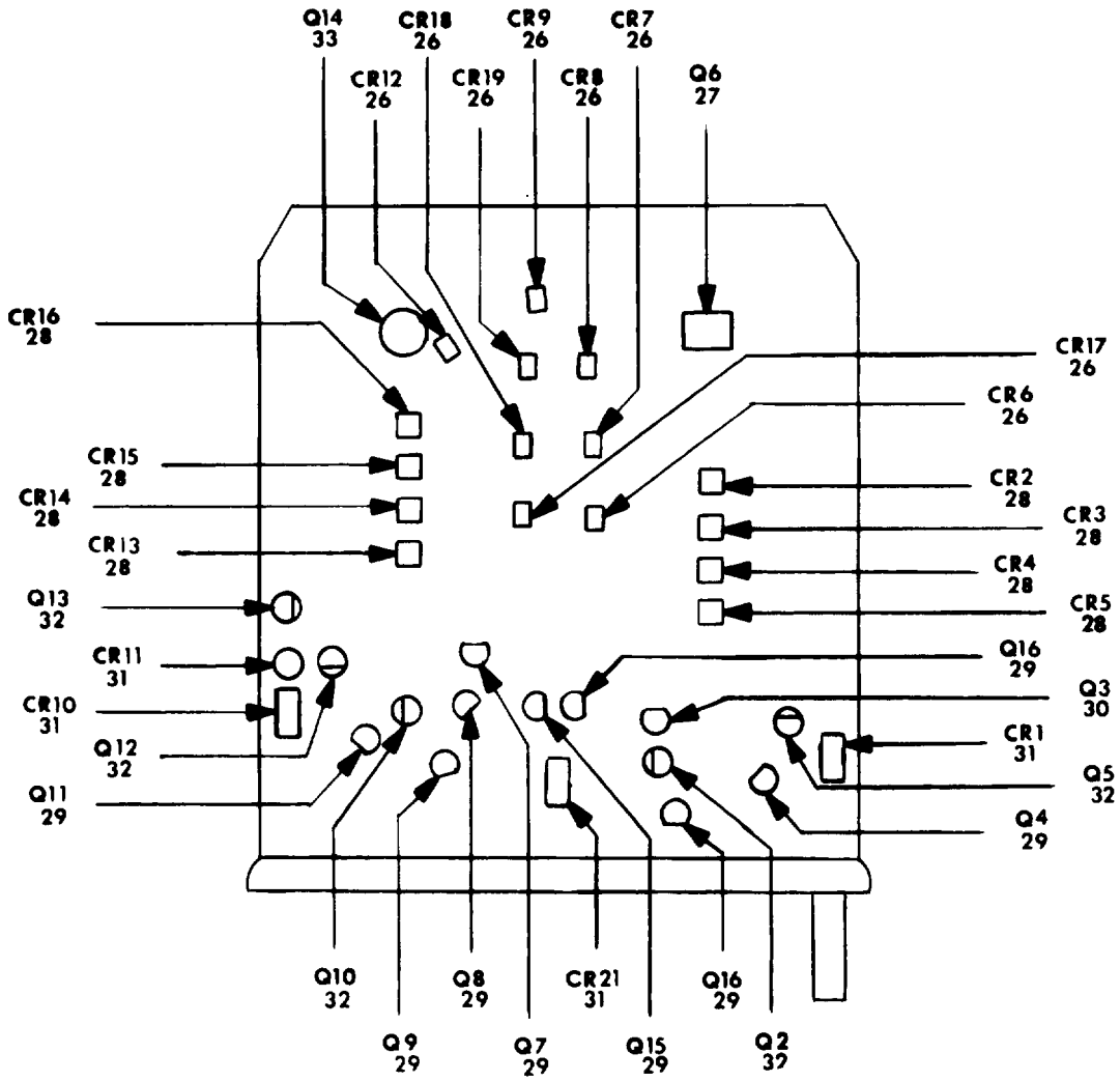
Figure 2-9. Module M19H (Sheet 3 of 7).
