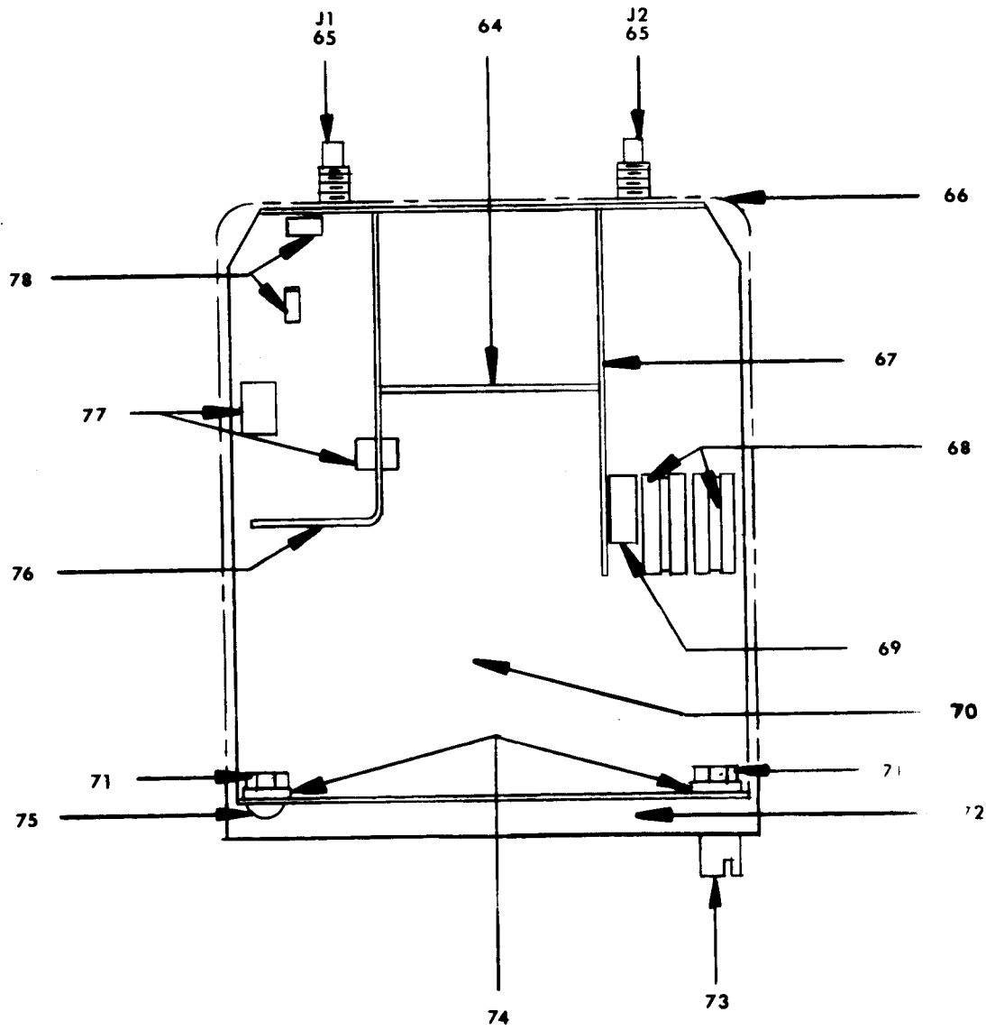
Figure 2-8. Module M10H (Sheet 6 of 7).
