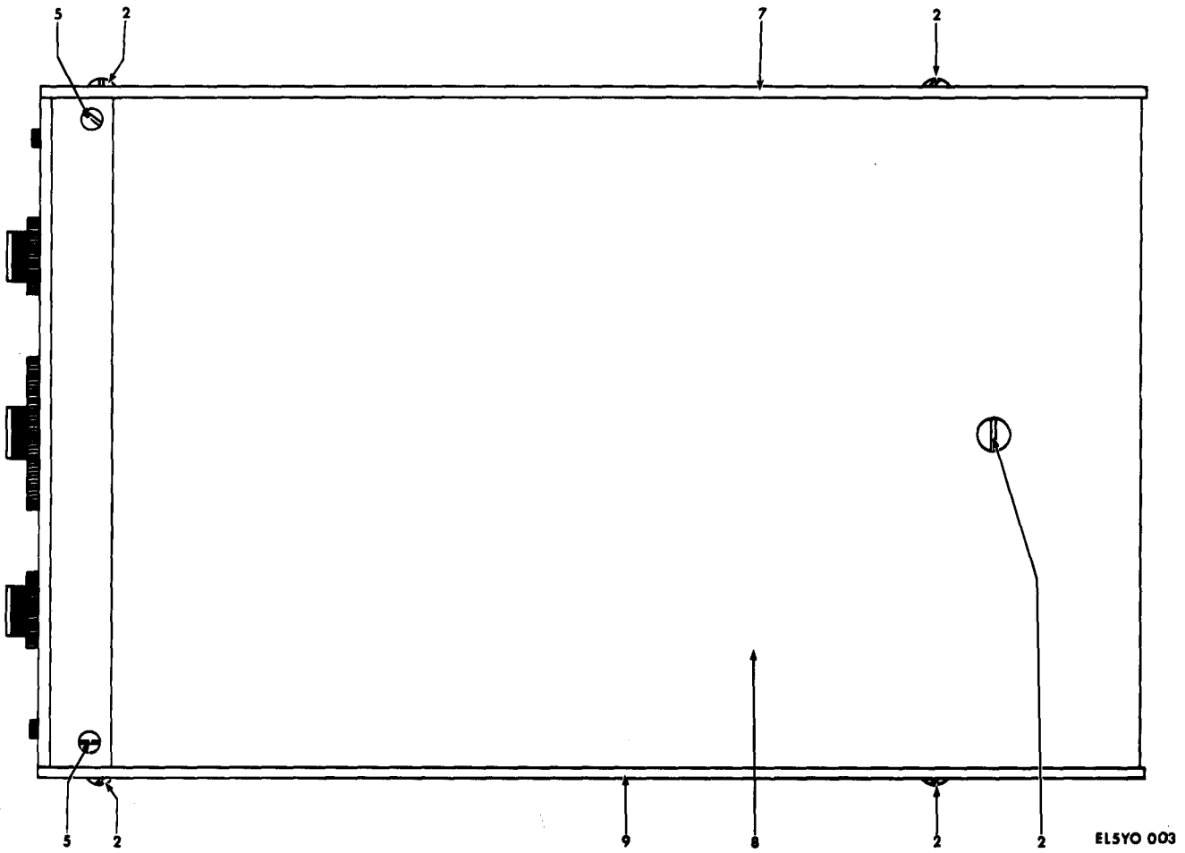
Figure 2-2. Sweep Generator SG-677A/U, Cabinet Assembly, (Sheet 2 of 2).
