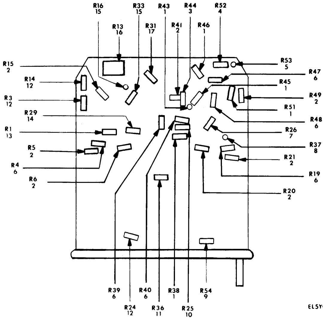
Figure 2-7. Module M9H (Sheet 1 of 5).
