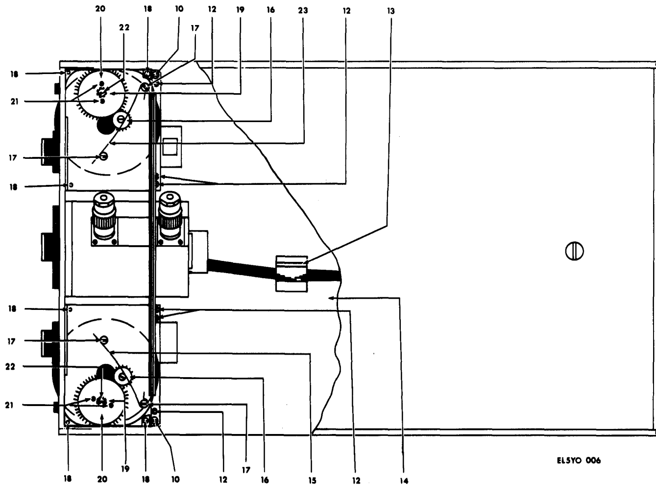
Figure 2-2. Sweep Generator SG-677A/U, Chassis Assembly, (Sheet 3 of 6).
